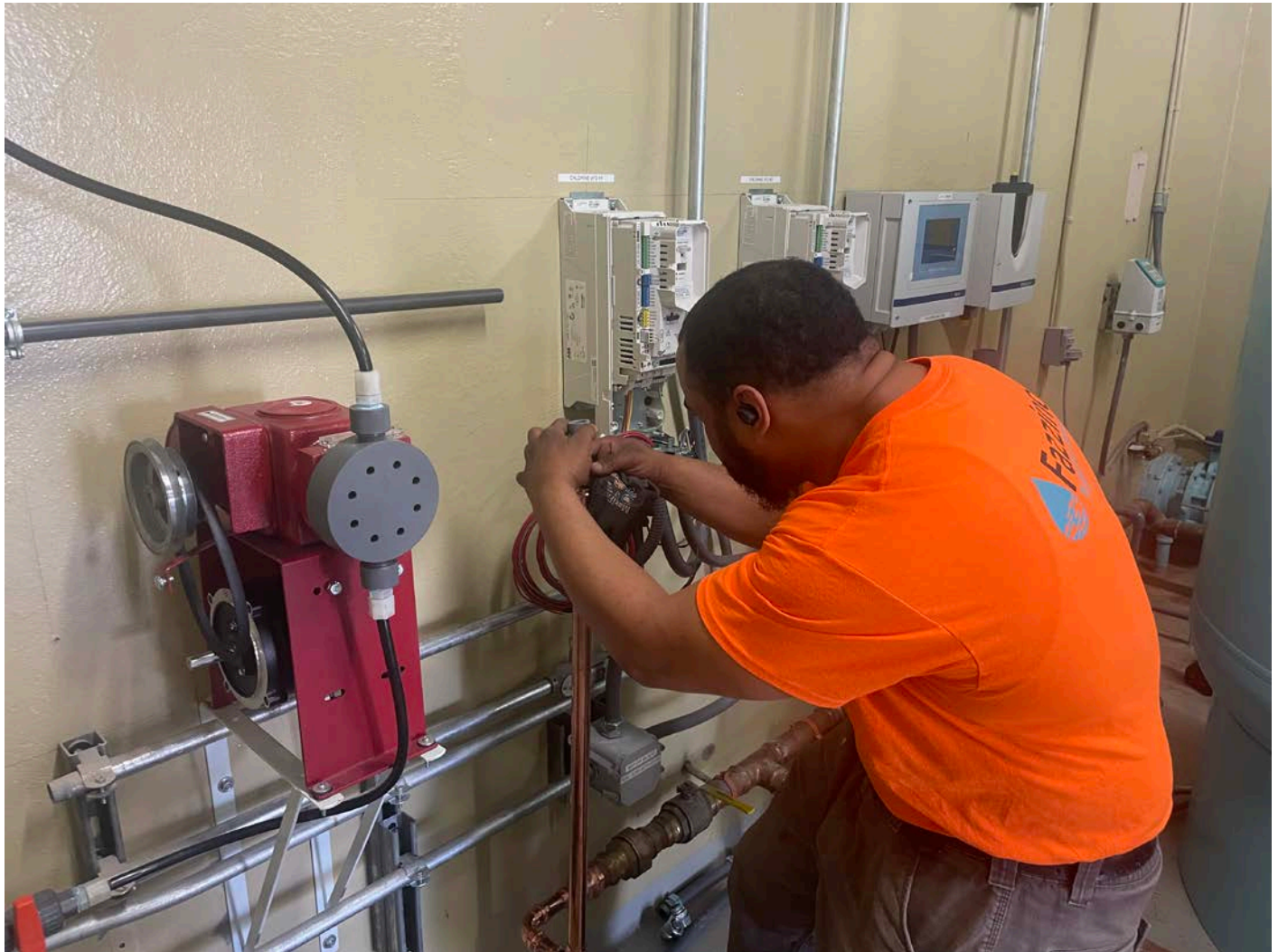
Picture 11: Fazzino Plumbing working on the installation of a chlorination system at the Long Hill Pump Station located on Long Hill Road in Middletown. View to the southwest.
